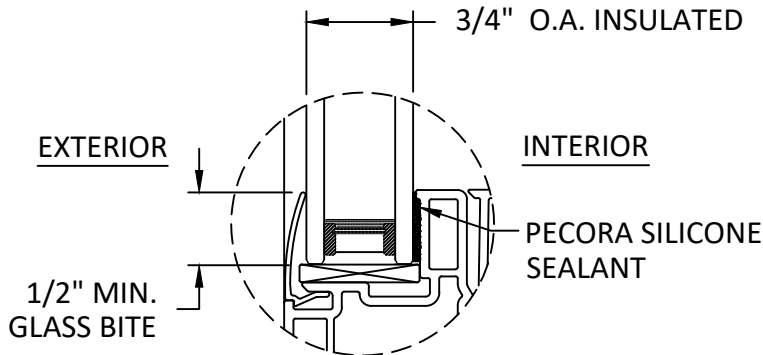
GLAZING DETAIL 1
