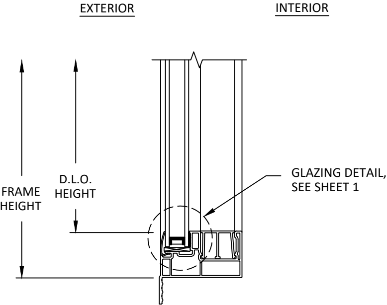
EXTERIOR INTERIOR D 4 VERTICAL SECTION V101 SILL
