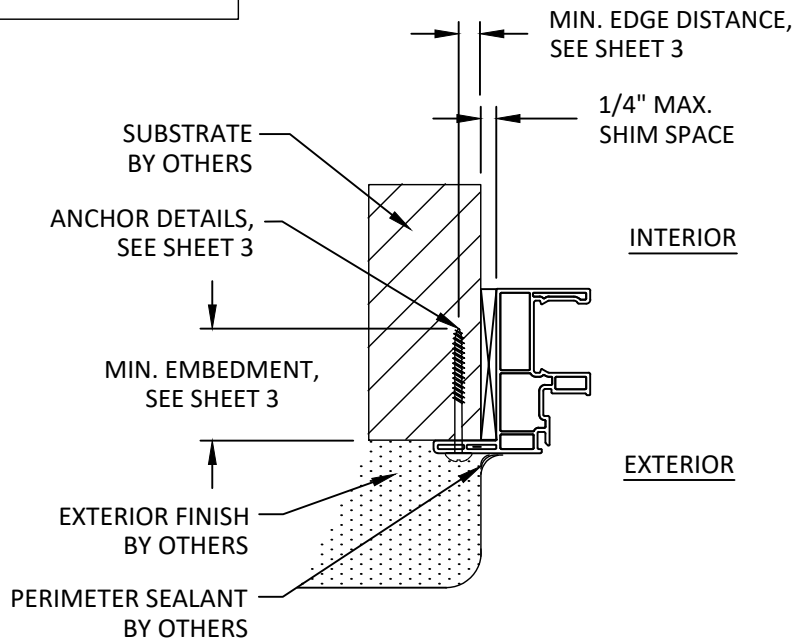
A 6 HORIZONTAL SECTION V152 JAMB NAIL FIN INSTALLATION
