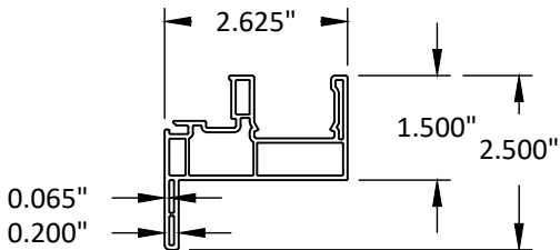
1 V152 FRAME HEAD/SILL/JAMB
