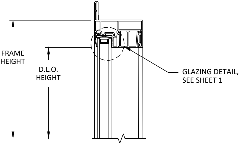
EXTERIOR INTERIOR C 4 VERTICAL SECTION V152 HEAD
